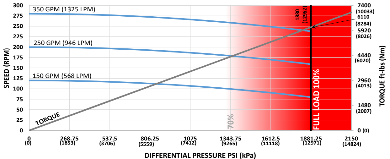
5 in (127mm) 6-7 Lobe 8.0 Stage HR
