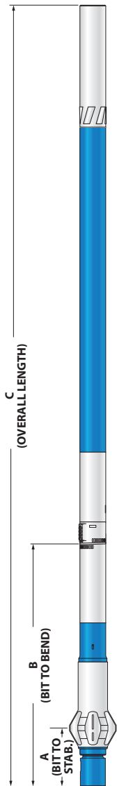
ADJUSTABLE BUILD RATE: 9-5/8 in (244 mm) Bottom w/ 8 in (203 mm) 7-8 Lobe 5.9 Stage HR SERIES 1
