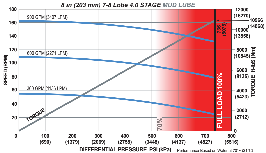
ADJUSTABLE BUILD RATE: 8 in (203 mm) 7-8 Lobe 4.0 Stage MUD LUBE
