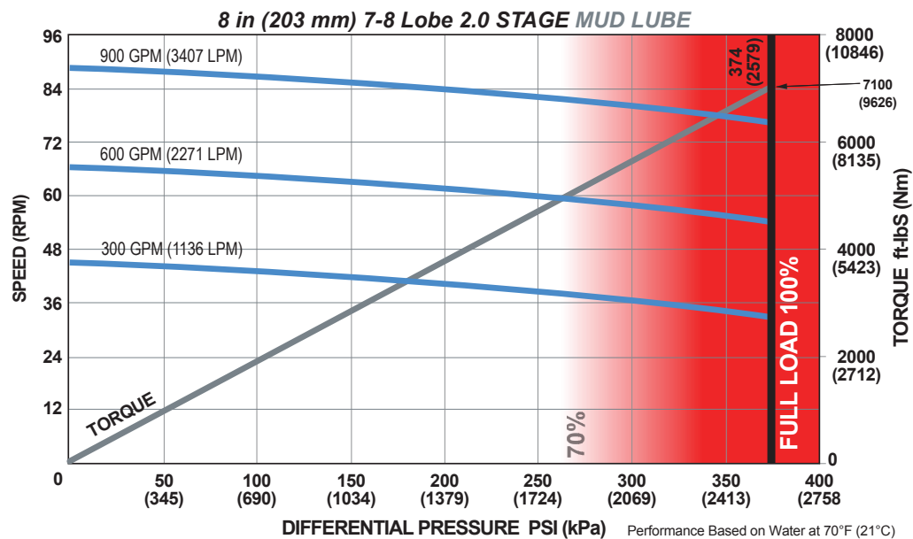
ADJUSTABLE BUILD RATE: 8 in (203 mm) 7-8 Lobe 2.0 Stage MUD LUBE
