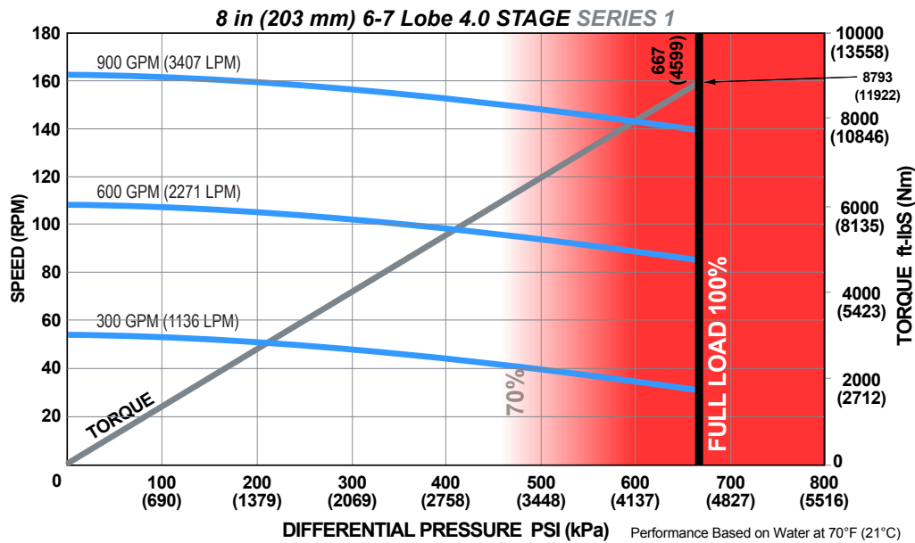
ADJUSTABLE BUILD RATE: 8 in (203 mm) 6-7 Lobe 4.0 Stage SERIES 1
