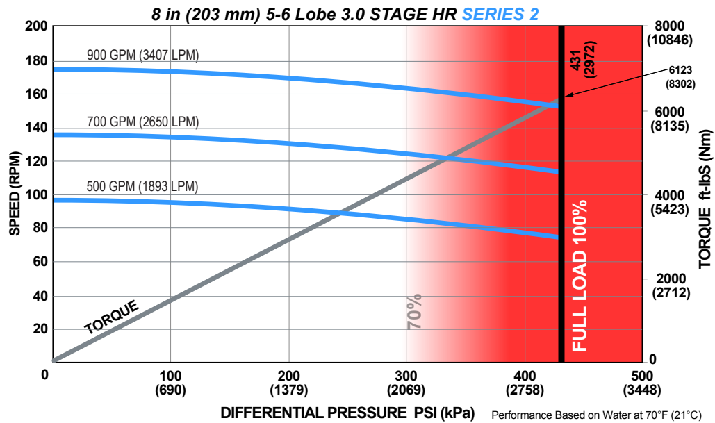
ADJUSTABLE BUILD RATE: 8 in (203 mm) 5-6 Lobe 3.0 Stage HR SERIES 2
