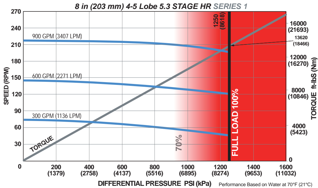
ADJUSTABLE BUILD RATE: 8 in (203 mm) 4-5 Lobe 5.3 Stage HR SERIES 1
