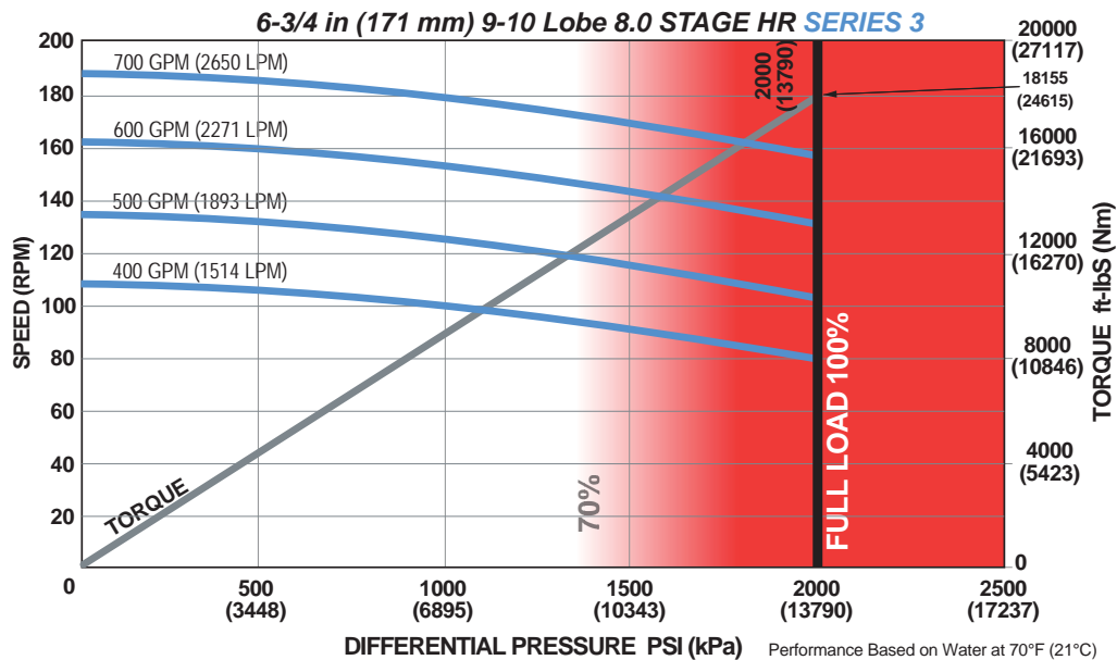
ADJUSTABLE BUILD RATE: 7 in (178 mm) Bottom w/ 6-3/4 (171 mm) 9-10 Lobe 8.0 Stage HR SERIES 3
