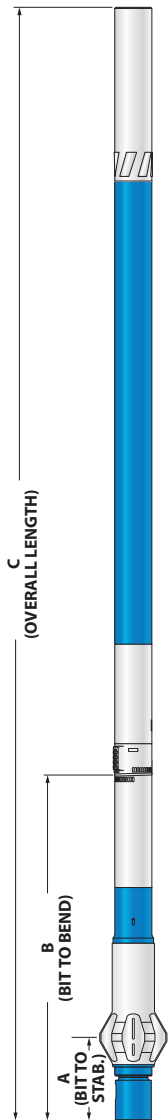
ADJUSTABLE BUILD RATE: 7 in (178 mm) Bottom w/ 6-3/4 (171 mm) 9-10 Lobe 8.0 Stage HR SERIES 3
