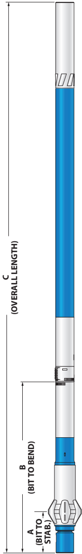
ADJUSTABLE BUILD RATE: 6 1/2 & 6 3/4 in (165 & 171 mm) 4-5 Lobe 7.0 Stage HR SERIES 1
