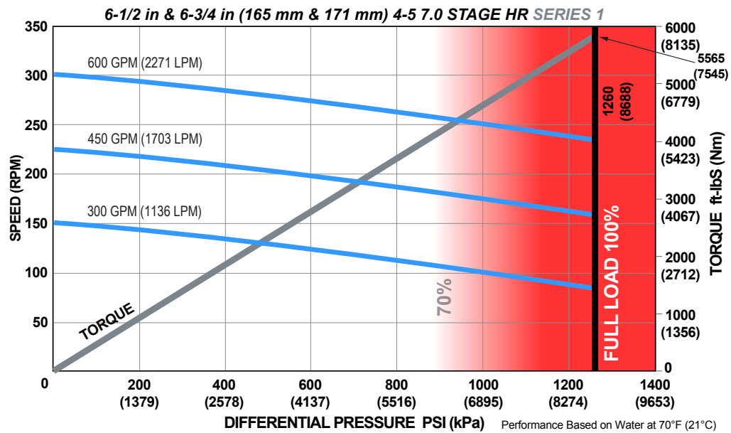
ADJUSTABLE BUILD RATE: 6 1/2 & 6 3/4 in (165 & 171 mm) 4-5 Lobe 7.0 Stage HR SERIES 1
