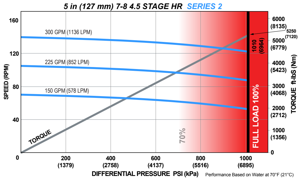
ADJUSTABLE BUILD RATE: 5 in (127 mm) 7-8 Lobe 4.5 Stage HR SERIES 2
