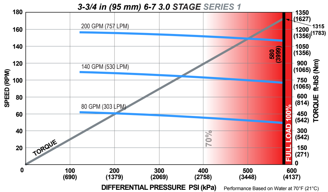
ADJUSTABLE BUILD RATE: 3 3/4 in (95 mm) 6-7 Lobe 3.0 Stage SERIES 1
