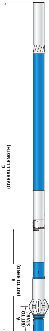
ADJUSTABLE BUILD RATE: 3 3/4 in (95 mm) 6-7 Lobe 3.0 Stage SERIES 1
