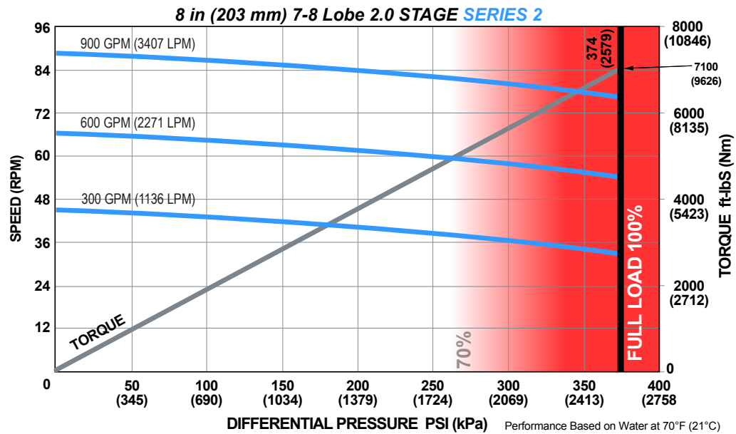
ADJUSTABLE BUILD RATE: 8 in (203 mm) 7-8 Lobe 2.0 Stage SERIES 2
