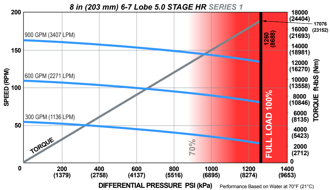
ADJUSTABLE BUILD RATE: 8 in (203 mm) 6-7 Lobe 5.0 Stage HR SERIES 1
