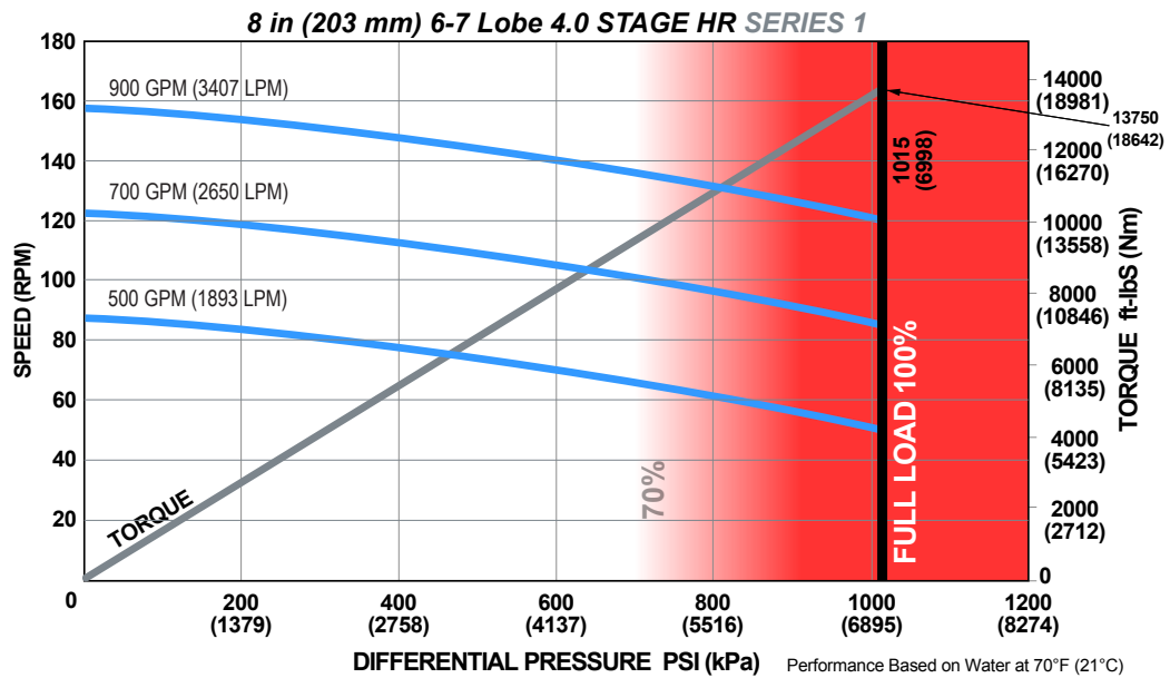
ADJUSTABLE BUILD RATE: 8 in (203 mm) 6-7 Lobe 4.0 Stage HR SERIES 1
