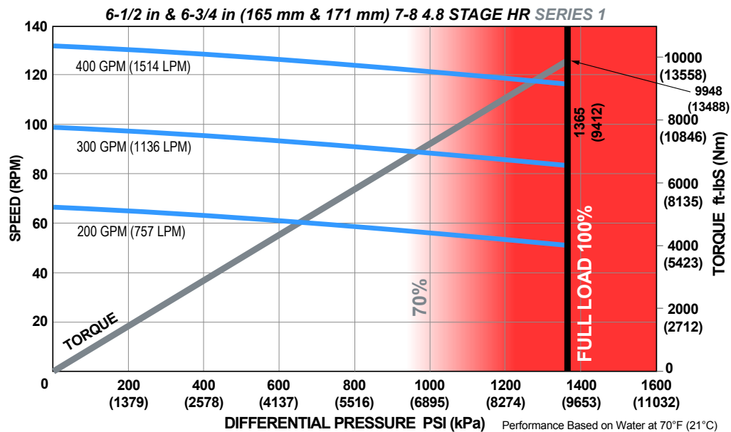
ADJUSTABLE BUILD RATE: 6 1/2 & 6 3/4 in (165 & 171 mm) 7-8 Lobe 4.8 Stage HR SERIES 1
