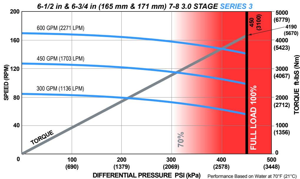
ADJUSTABLE BUILD RATE: 6-1/2 & 6-3/4 in (165 & 171 mm) 7-8 Lobe 3.0 Stage SERIES 3
