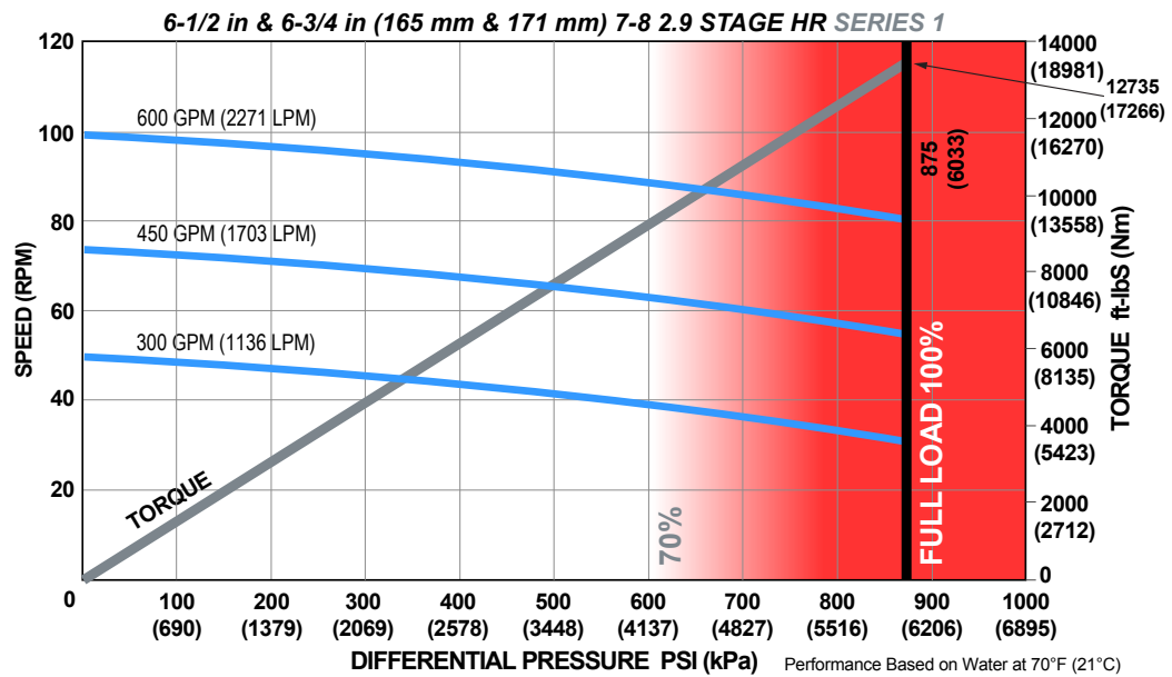
ADJUSTABLE BUILD RATE: 6 1/2 & 6 3/4 in (165 & 171 mm) 7-8 Lobe 2.9 Stage HR SERIES 1
