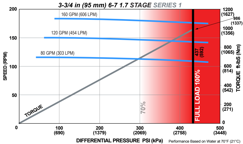
ADJUSTABLE BUILD RATE: 3 3/4 in (95 mm) 6-7 Lobe 1.7 Stage SERIES 1
